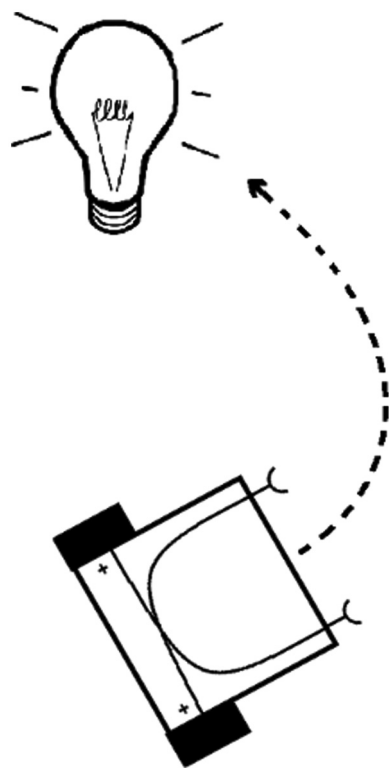
Figure 1. A Braitenberg vehicle is a little cart with two light sensitive sensors directly connected ipsilaterally to two motors driving the vehicle. This configuration makes the vehicle drive towards the light.
